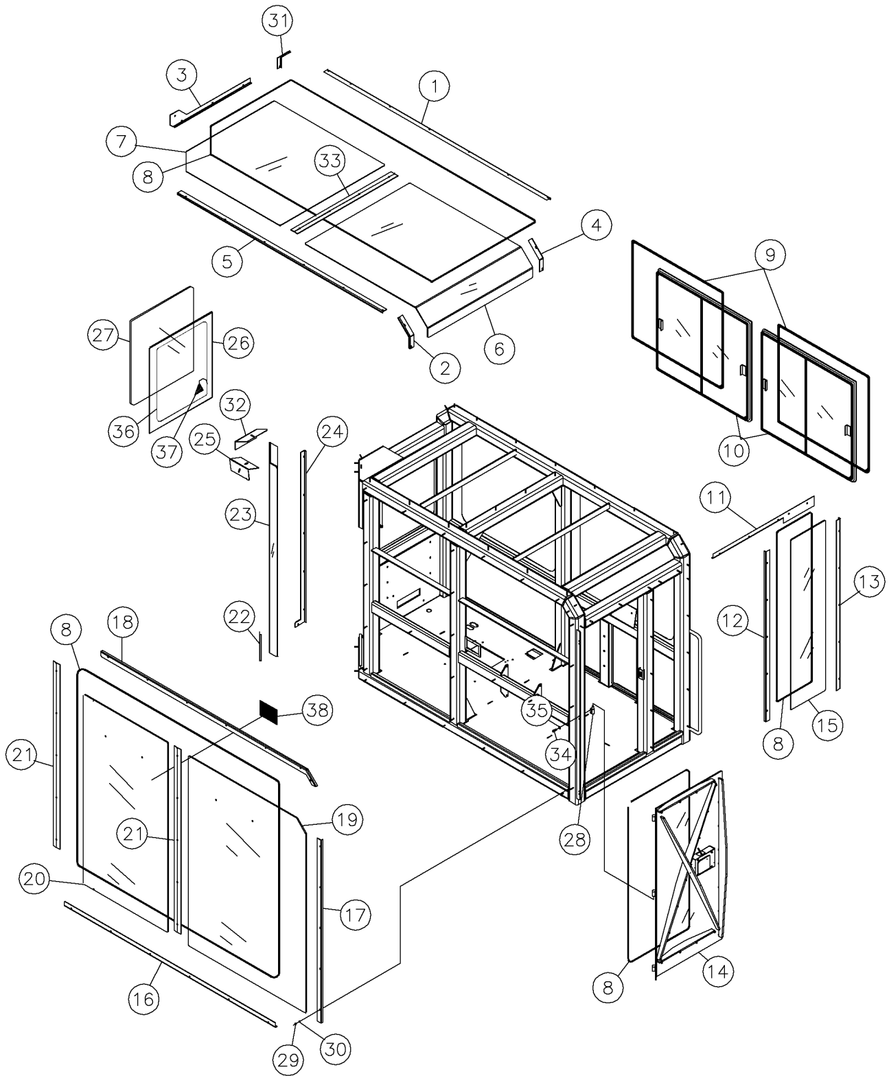
Cab Window Assy Fig 6-3
