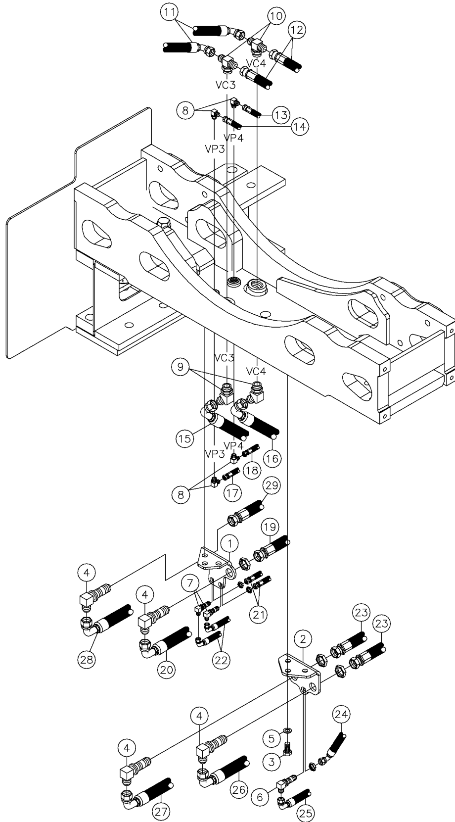
Vise Box Plumbing Assy S/N 105 & 107-110 Fig 8-3
