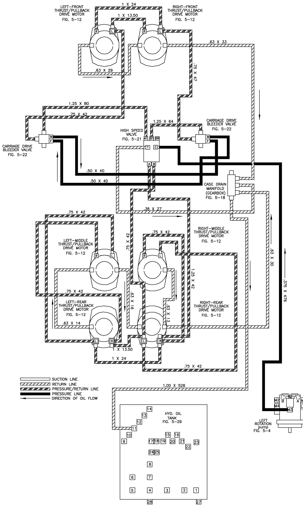
Diagram-Hyd Location-Thrust/Pullback Motors Fig 13-3r01
