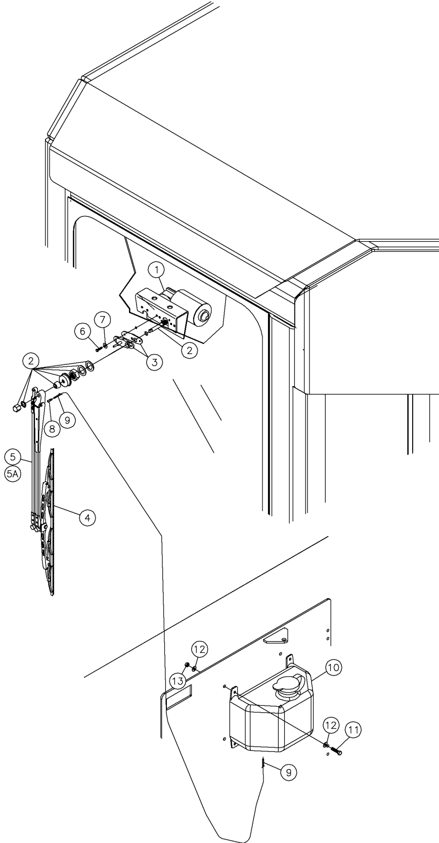
Cab-Wiper Motor Assy Fig 6-10r01
