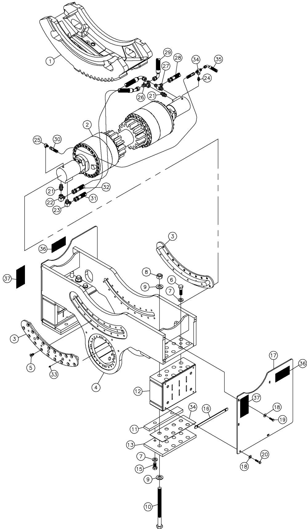
Vise Scissor Rotation Assy S/N 111- Fig 8-10r01
