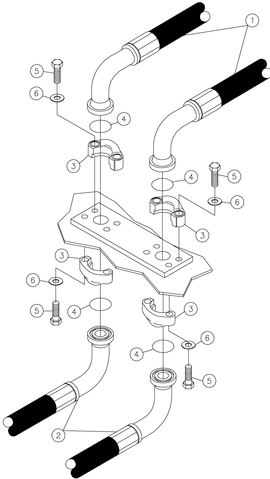
Hyd-Main Frame Manifold Fig 5-32
