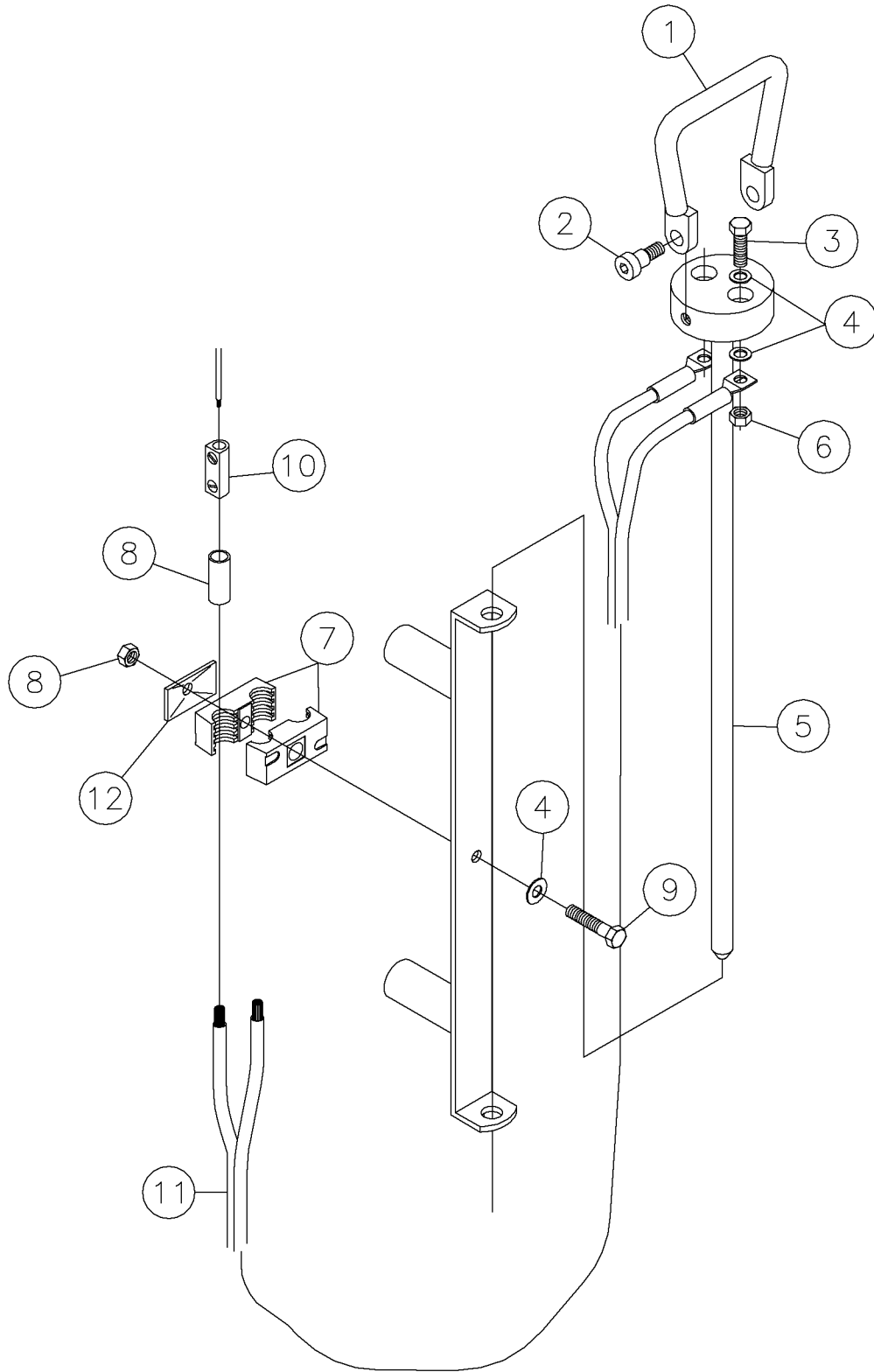
Safety-Voltage Stake Assy Fig 11-1r01
