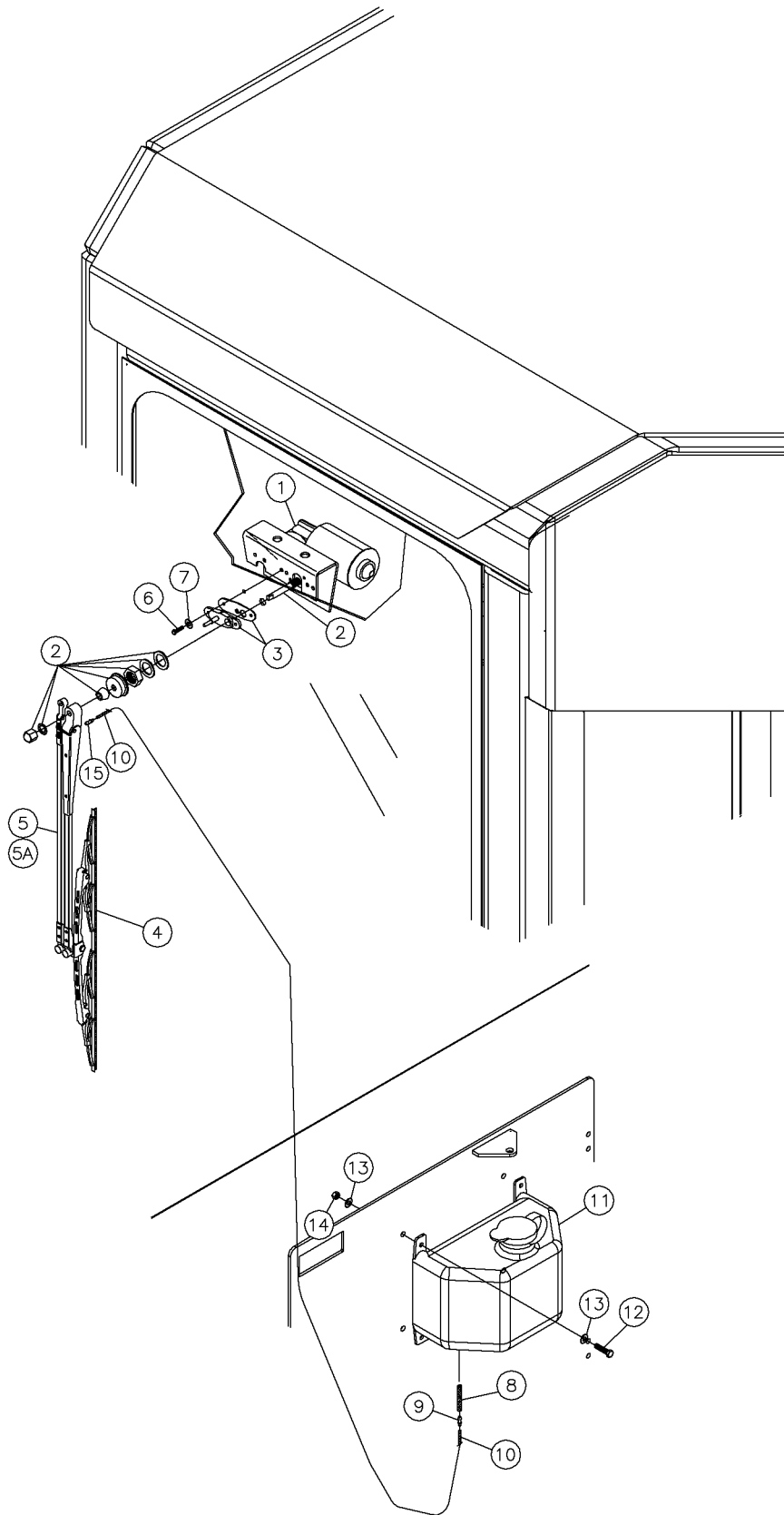
Cab-Wiper Motor Assy Fig 6-10
