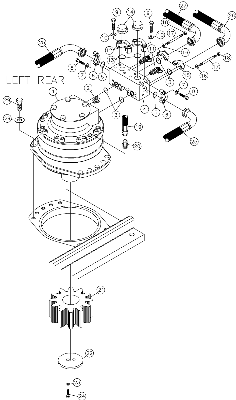
Hyd-Motor-Thrust/Pullback Drive Assy(LR) Fig 5-12x04
