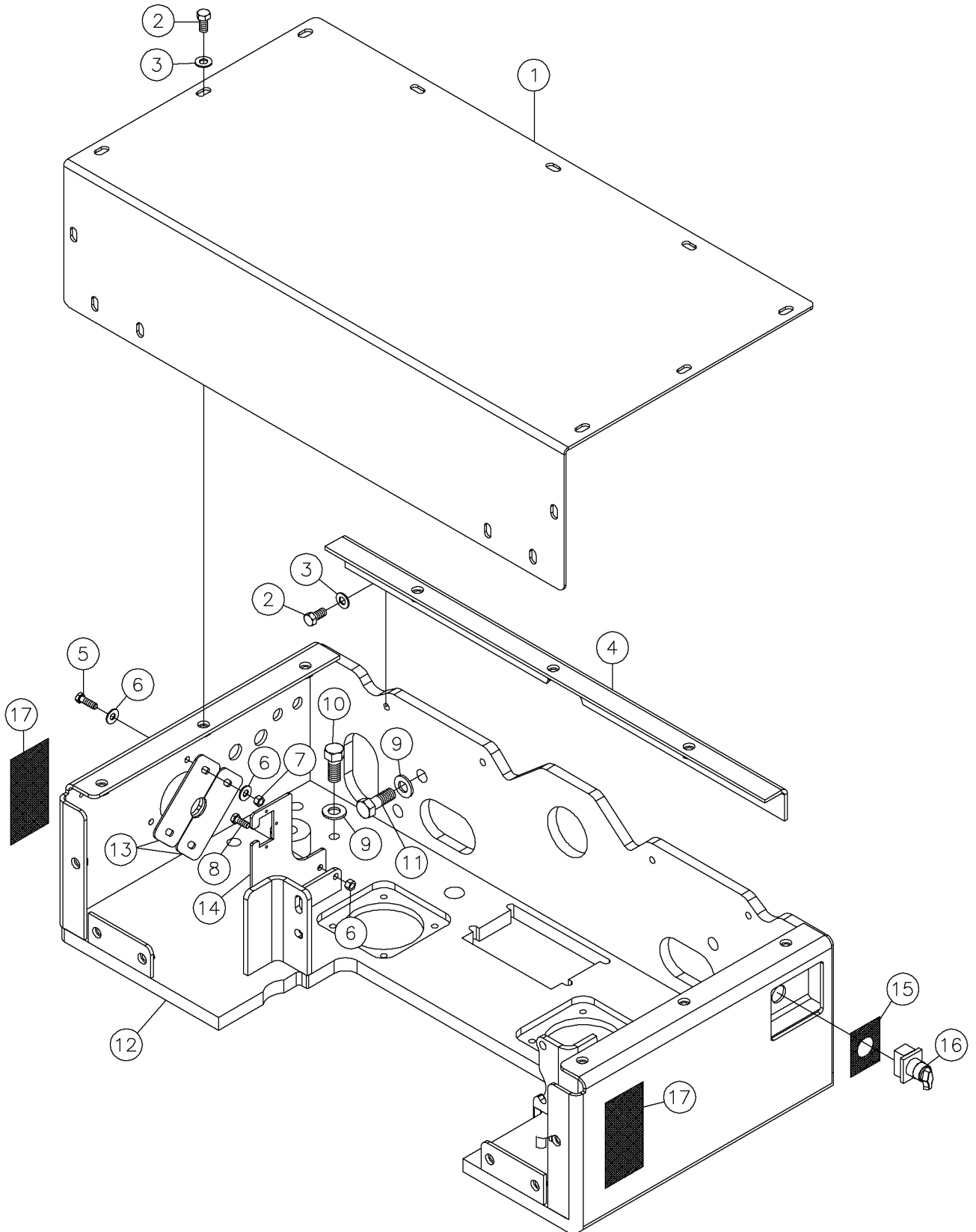
Vise Drive Frame Assy S/N 111- Fig 8-5r01
