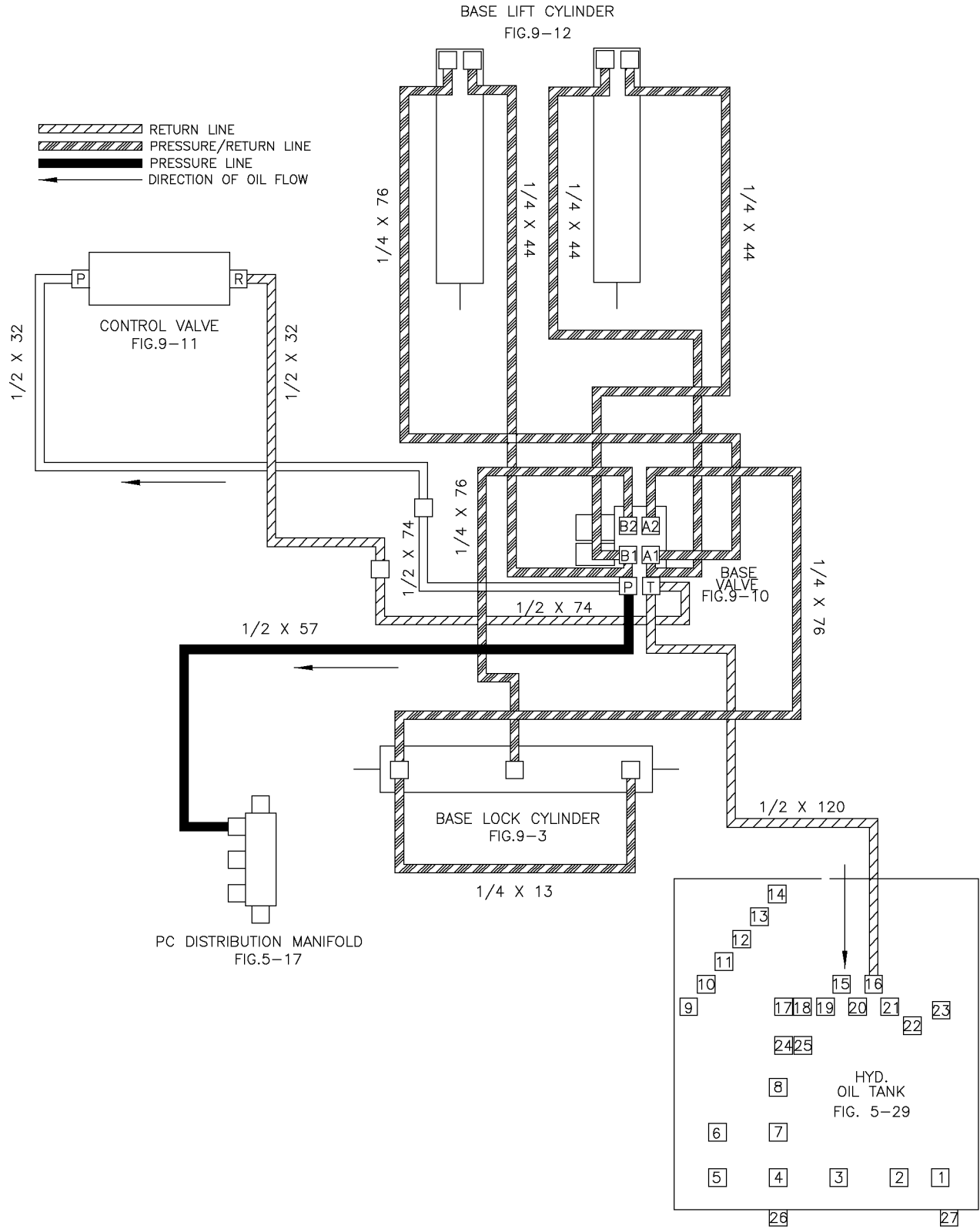
Diagram-Hyd Location-Crane Base Lift Fig 13-1r02
