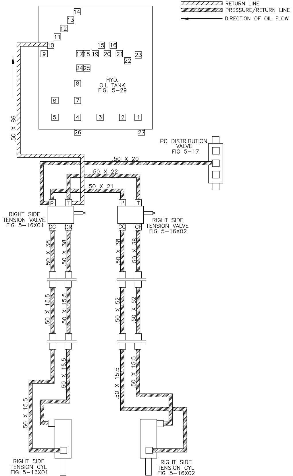
Diagram-Hyd Location Track Tension Valve/Cylinder Fig 13-11
