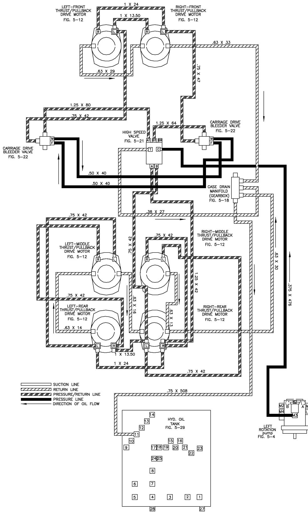
Diagram-Hyd Location-Thrust/Pullback Motors Fig 13-3
