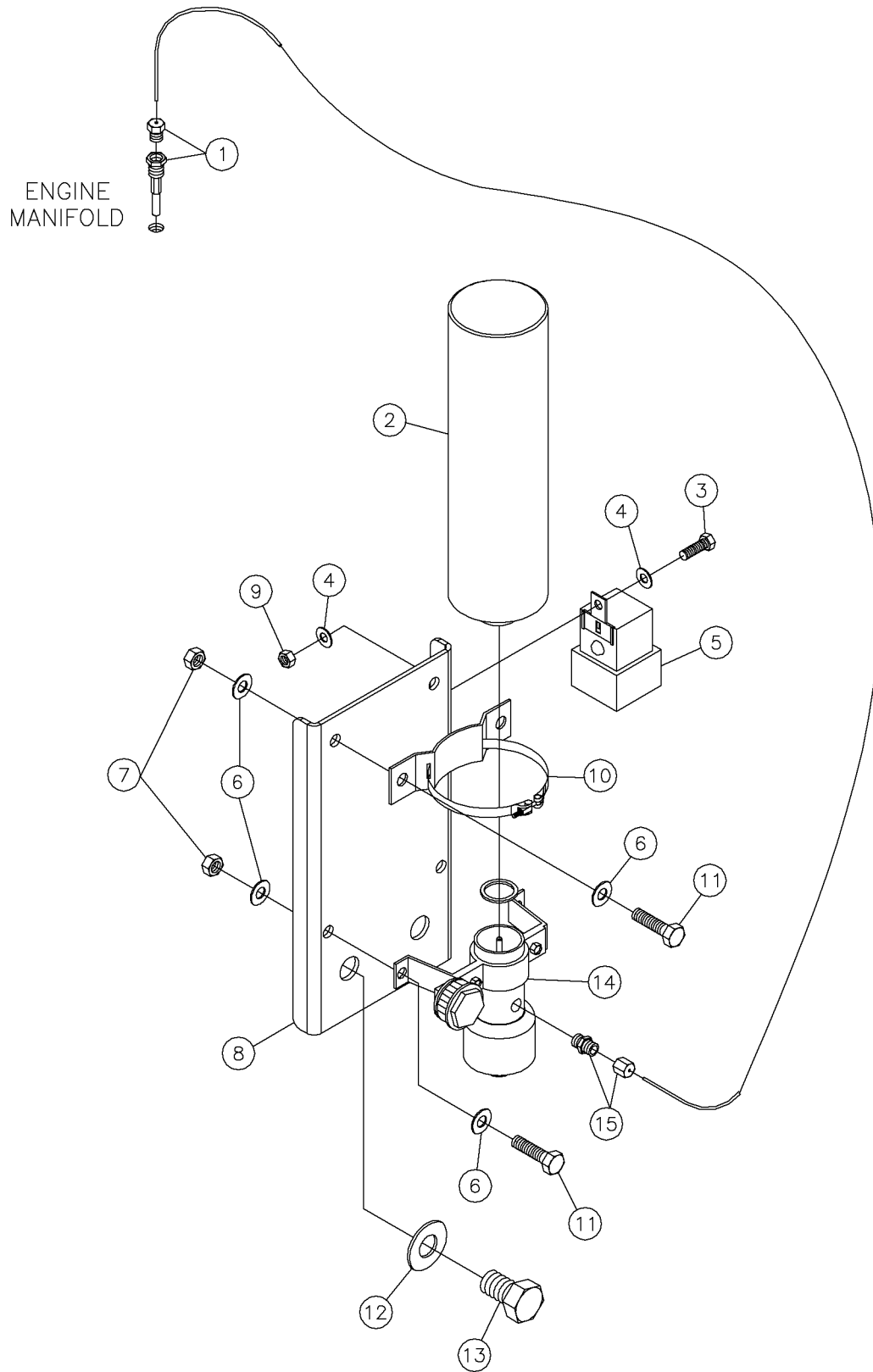
Engine - Ether Start Assy Fig 3-9
