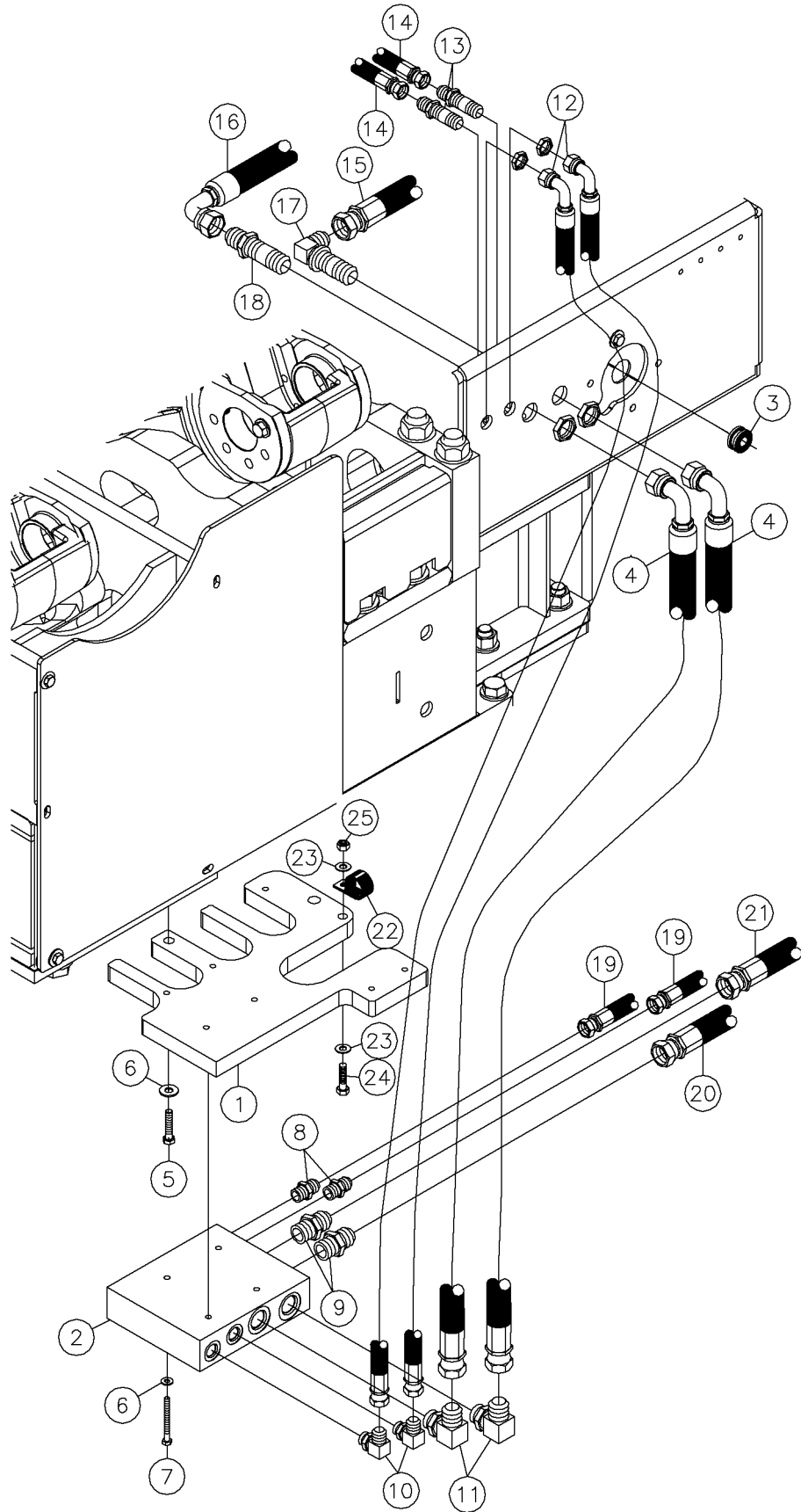
Vise Scissor Vise Manifold Assy S/N 111- Fig 8-14r01
