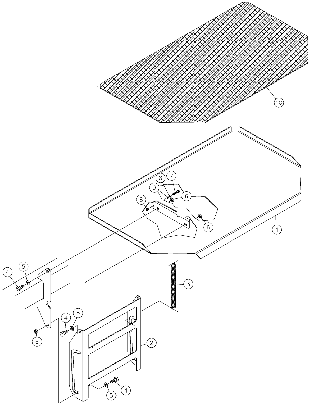
Cab-Side Table Assy Fig 6-8
