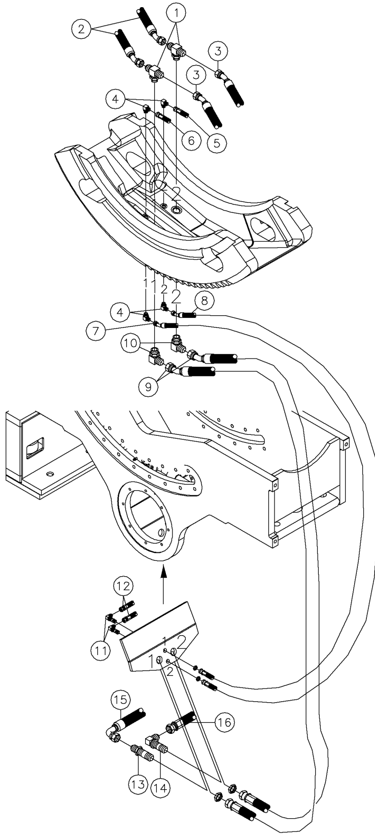
Vise Scissor Rotation Bulkhead Assy S/N 105 & 107-110 Fig 8-11
