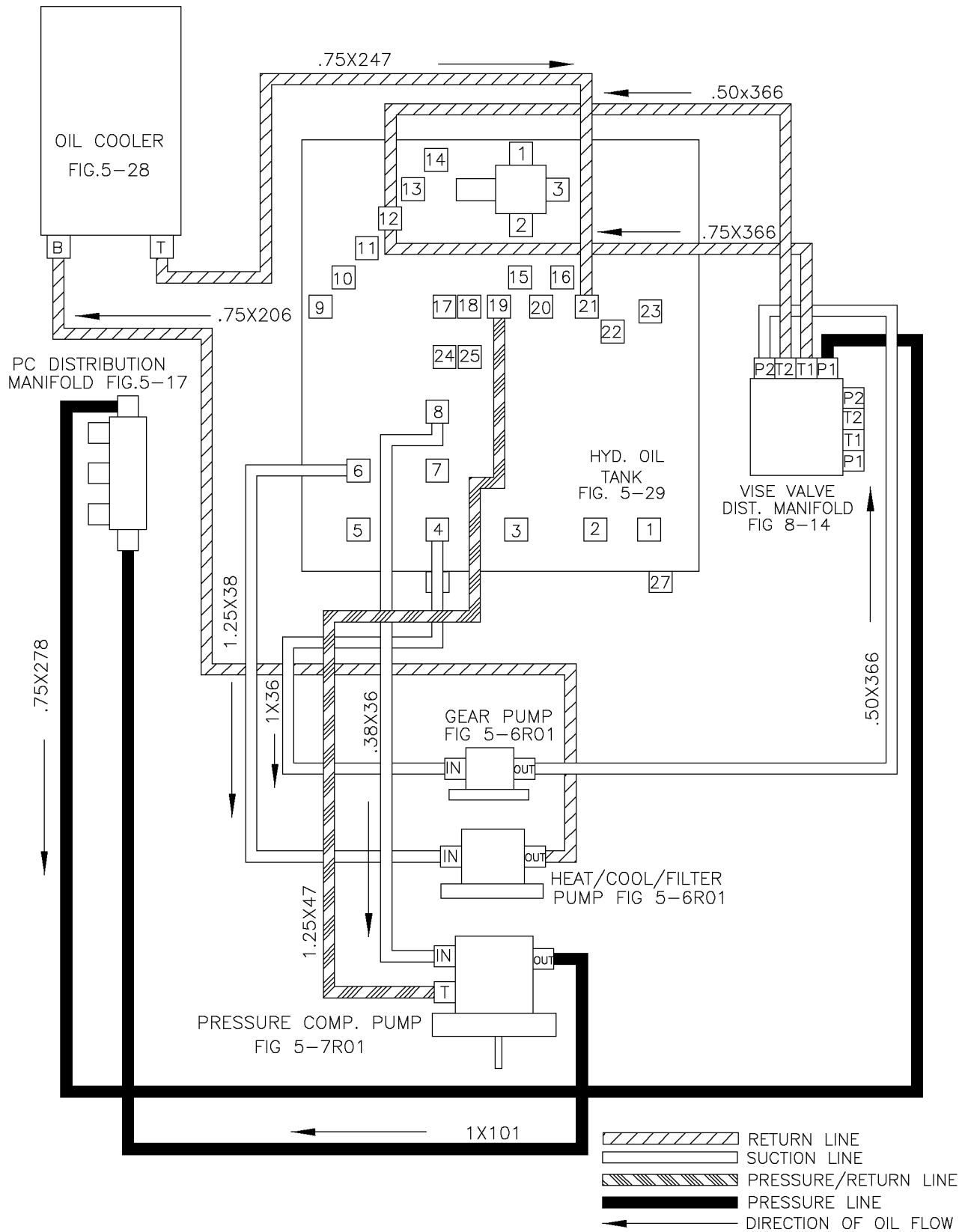
Diagram-Hyd Location Triple Stack Pump/Oil Cooler Fig 13-10r01
