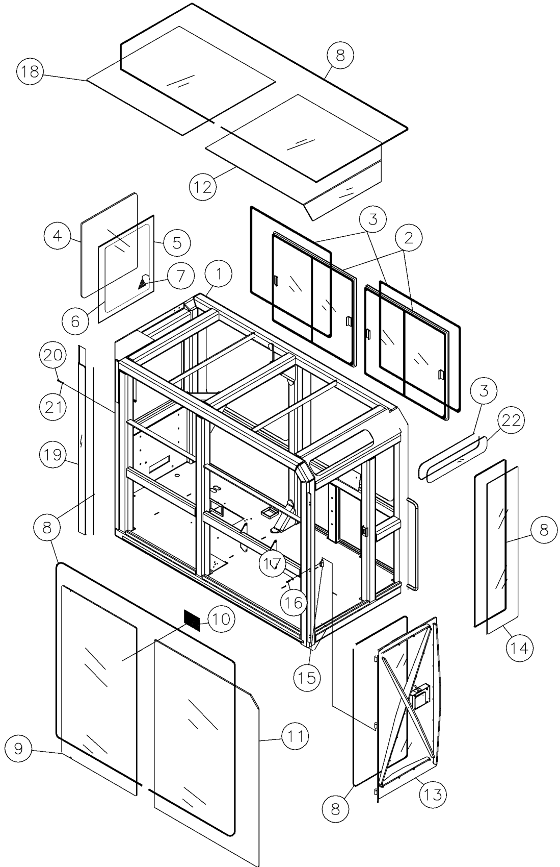
Cab Window Assy Fig 6-3r02
