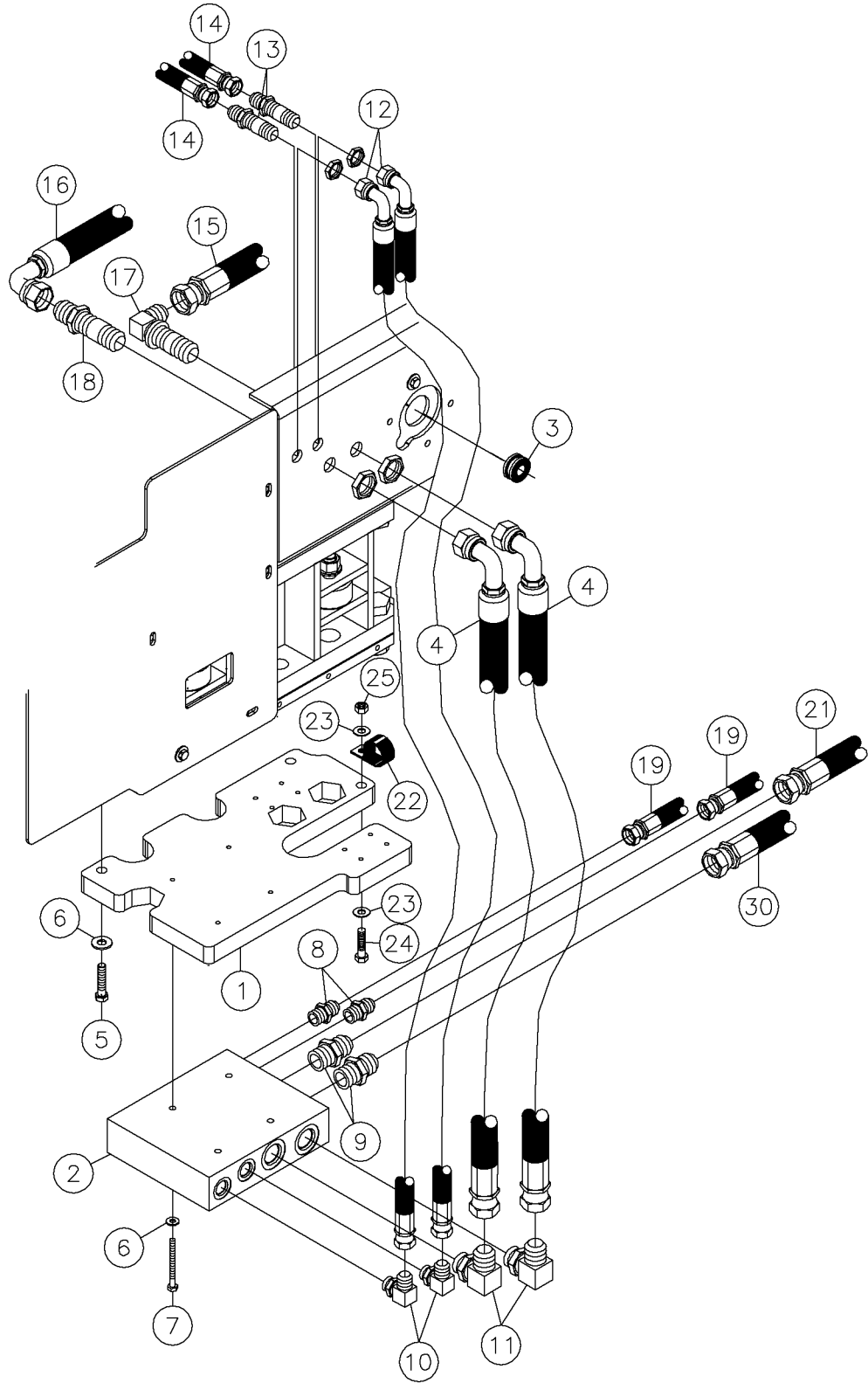
Vise Scissor Vise Manifold Assy S/N 105 & 107-110 Fig 8-14
