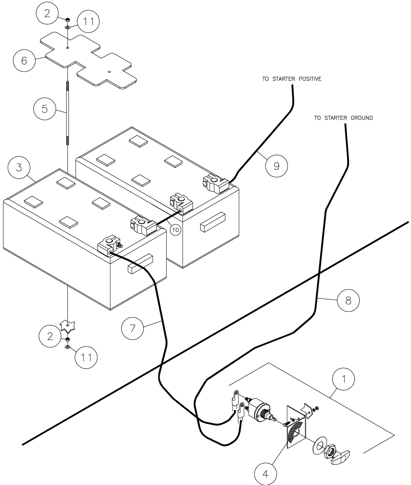
Control/Electrical- Battery Assy Fig 7-3
