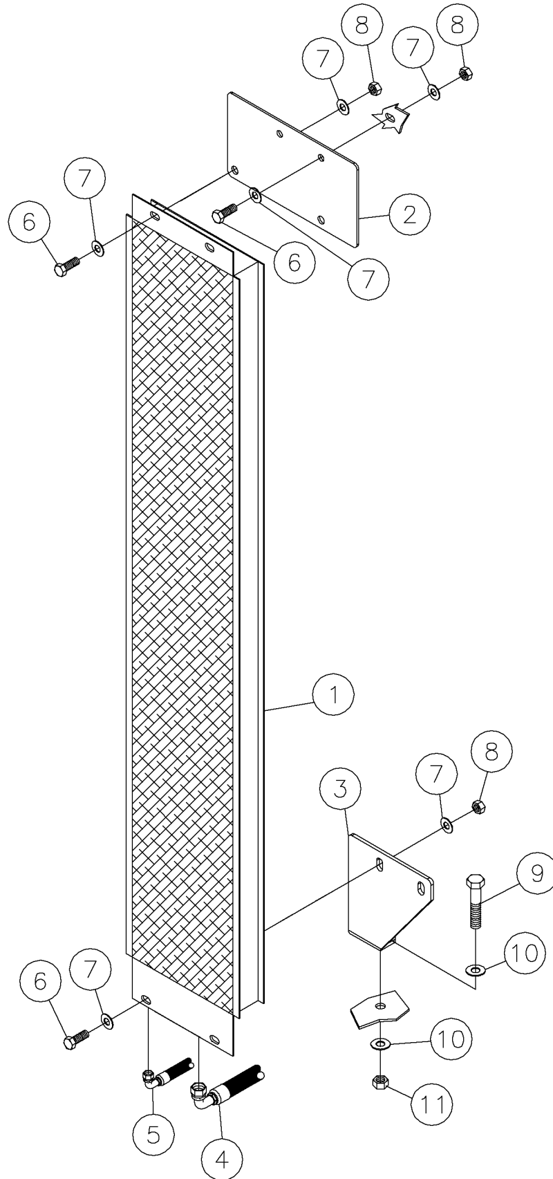
Cab-Air Conditioner Condenser Assy Fig 6-17
