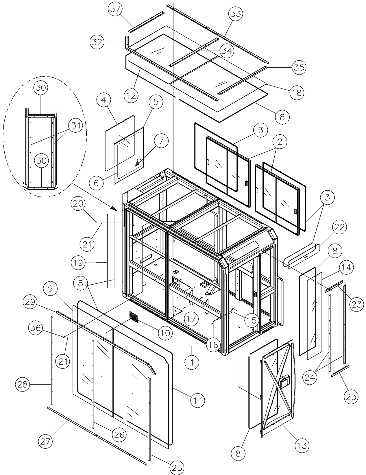
Cab Window Assy Fig 6-3r03
