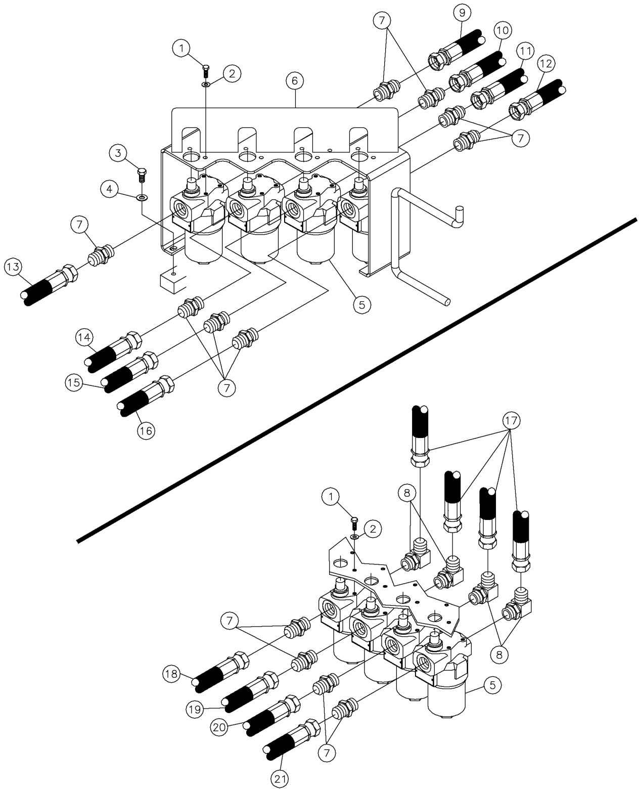
Hyd-High Pressure Filter Assy Fig 5-27
