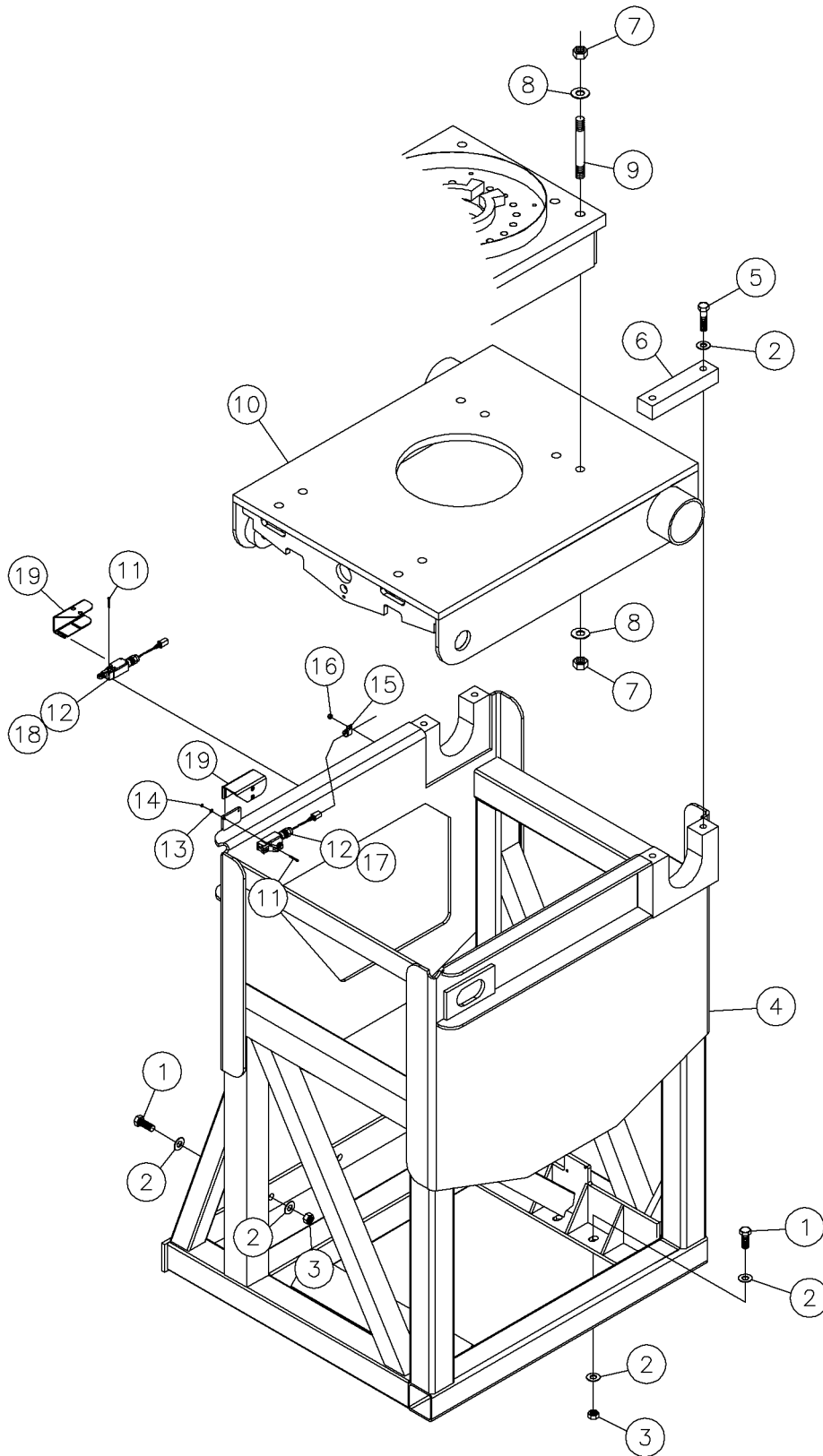
Cable Crane-Frame Assy Fig 9-2
