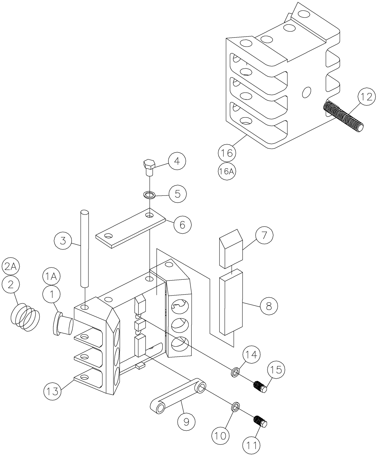
Component-Upper Jaw/Lower Jaw/Piston Jaw Assy Fig 12-40
