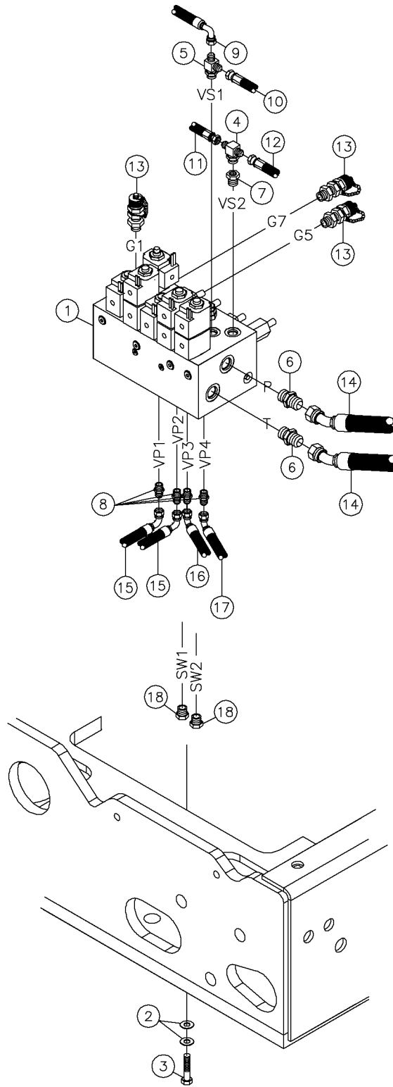
Vise Lift Valve Assy S/N 105 & 107-110 Fig 8-9
