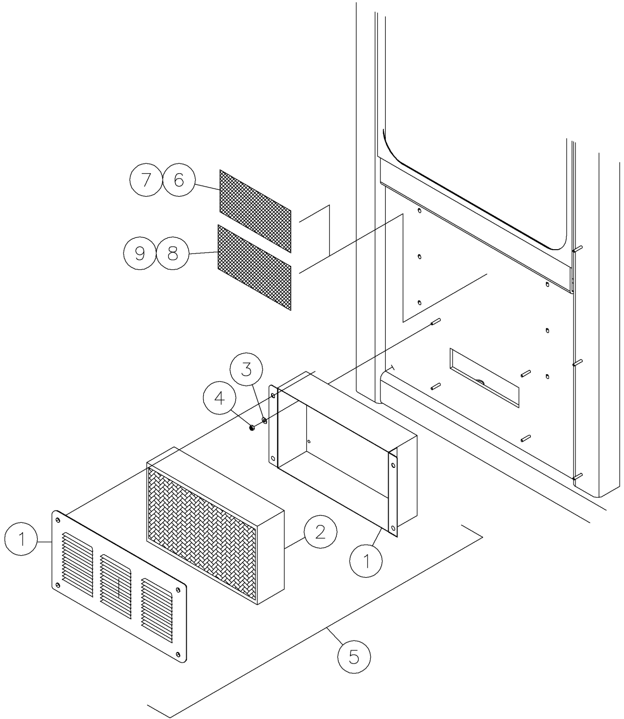
Cab-Air Conditioner Filter Assy Fig 6-14
