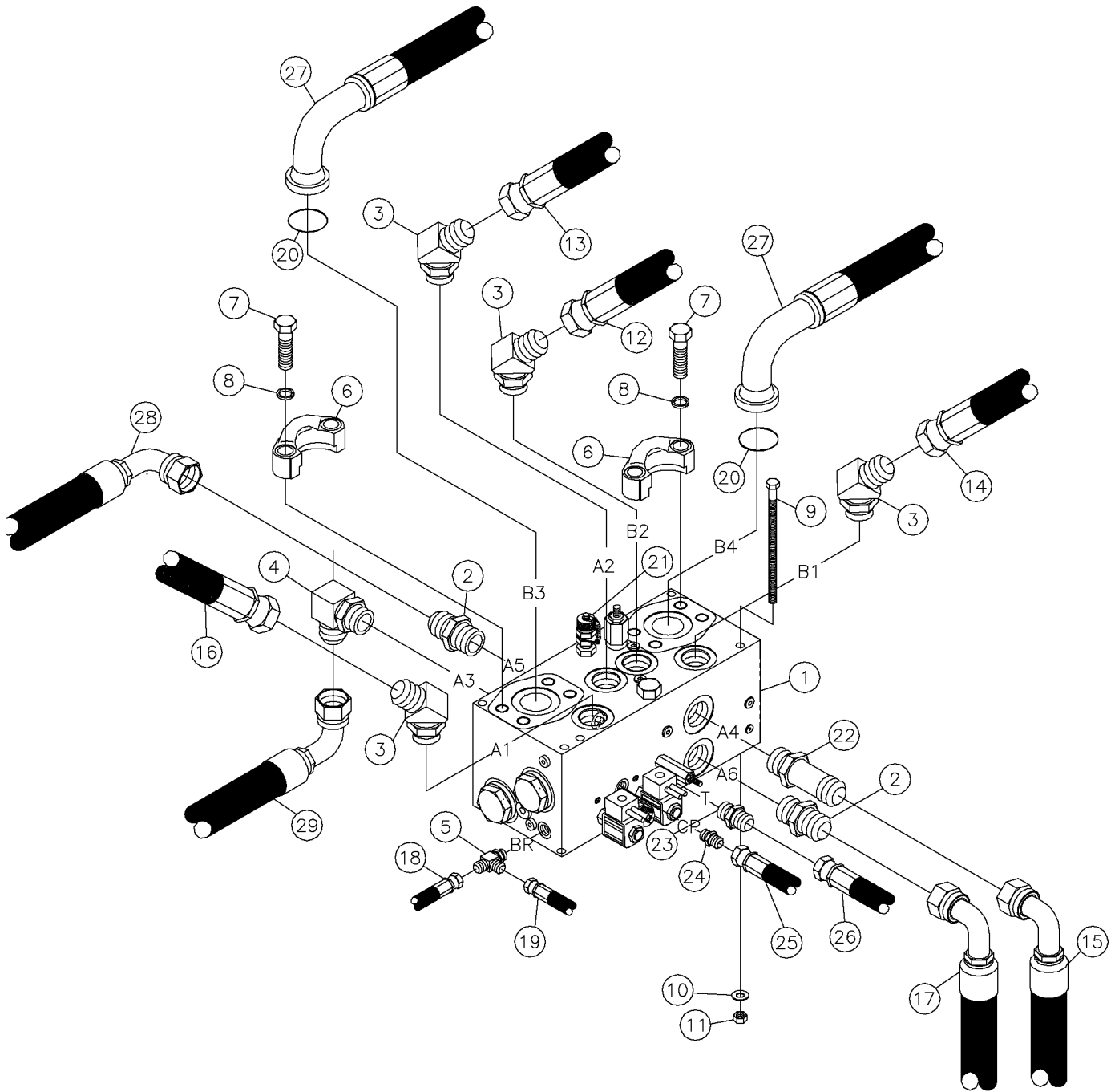
Hyd-Valve-Diverter Assy Fig 5-23r01
