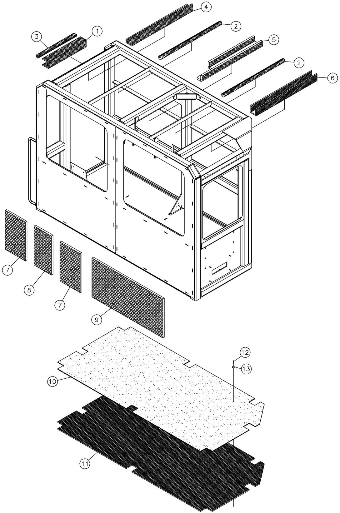
Cab-Foam Assy Fig 6-2r01
