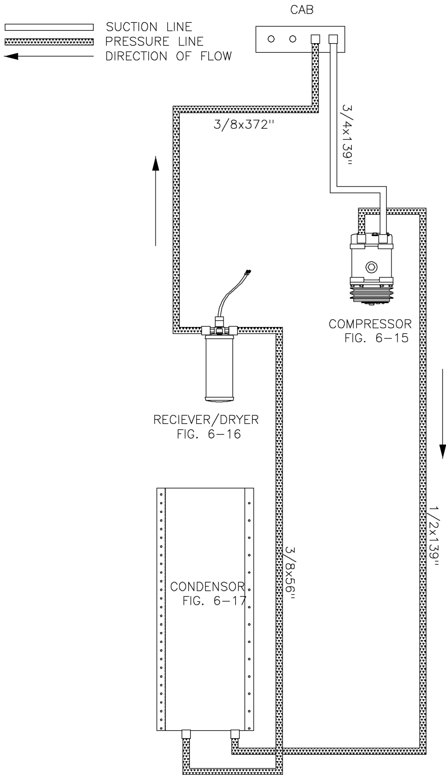
Cab-Air Conditioner Component Coolant Diagram Fig 6-12
