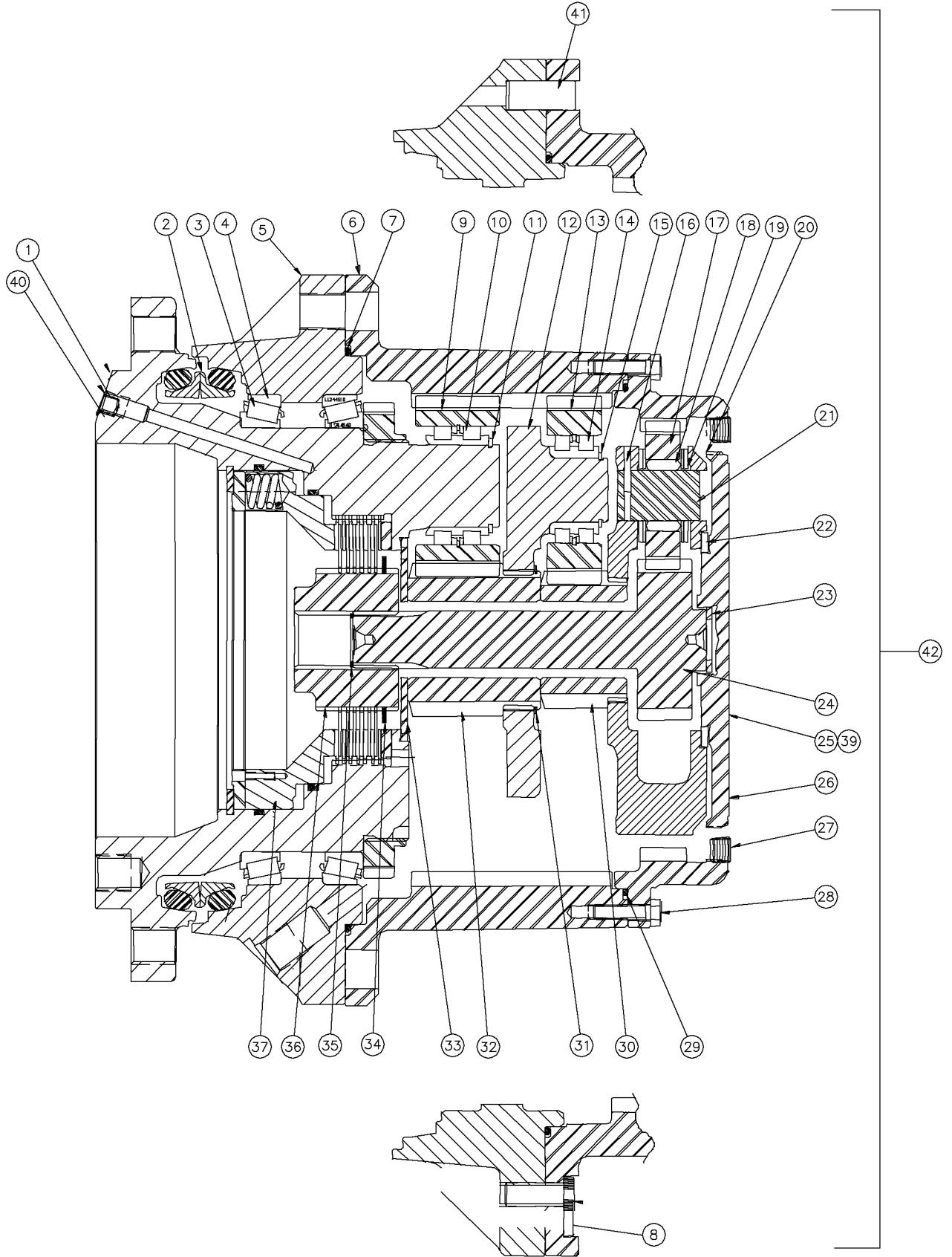
Component-Track Drive Gearbox Fig 12-22
