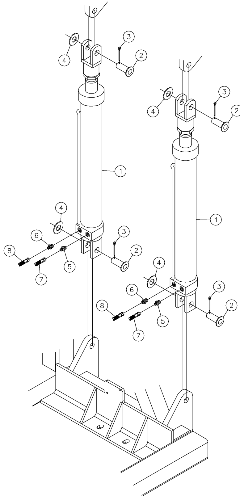
Crane Base Lift Cylinder Assy Fig 9-12
