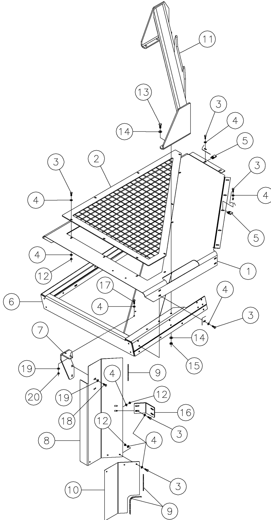
Shield-Radiator Top Assy Fig 4-2r02
