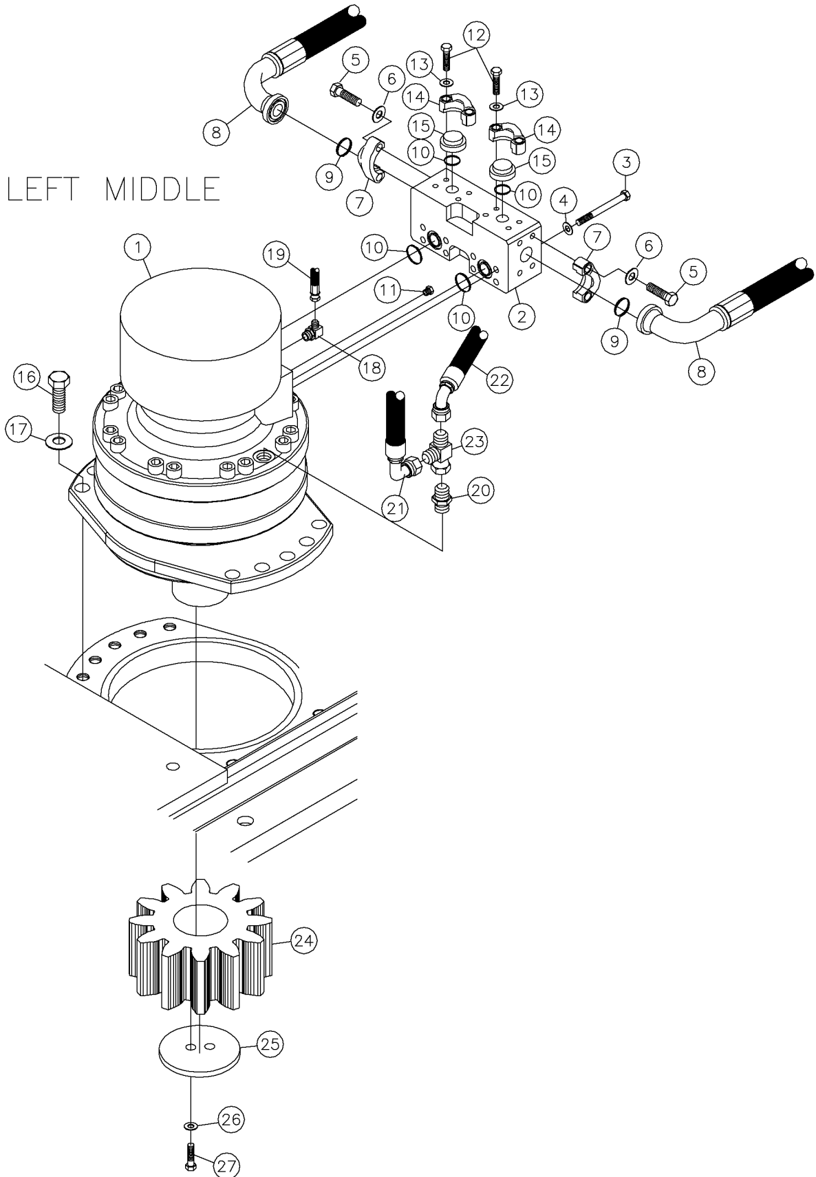
Hyd-Motor-Thrust/Pullback Drive Assy(LM) Fig 5-12x02
