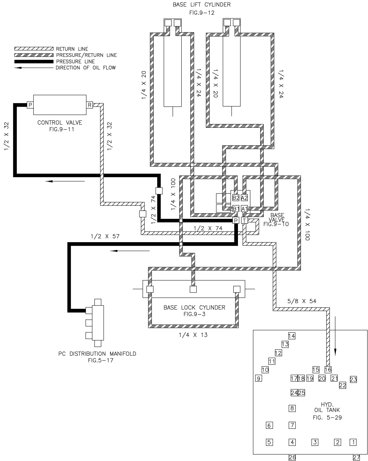
Diagram-Hyd Location-Crane Base Lift Fig 13-1
