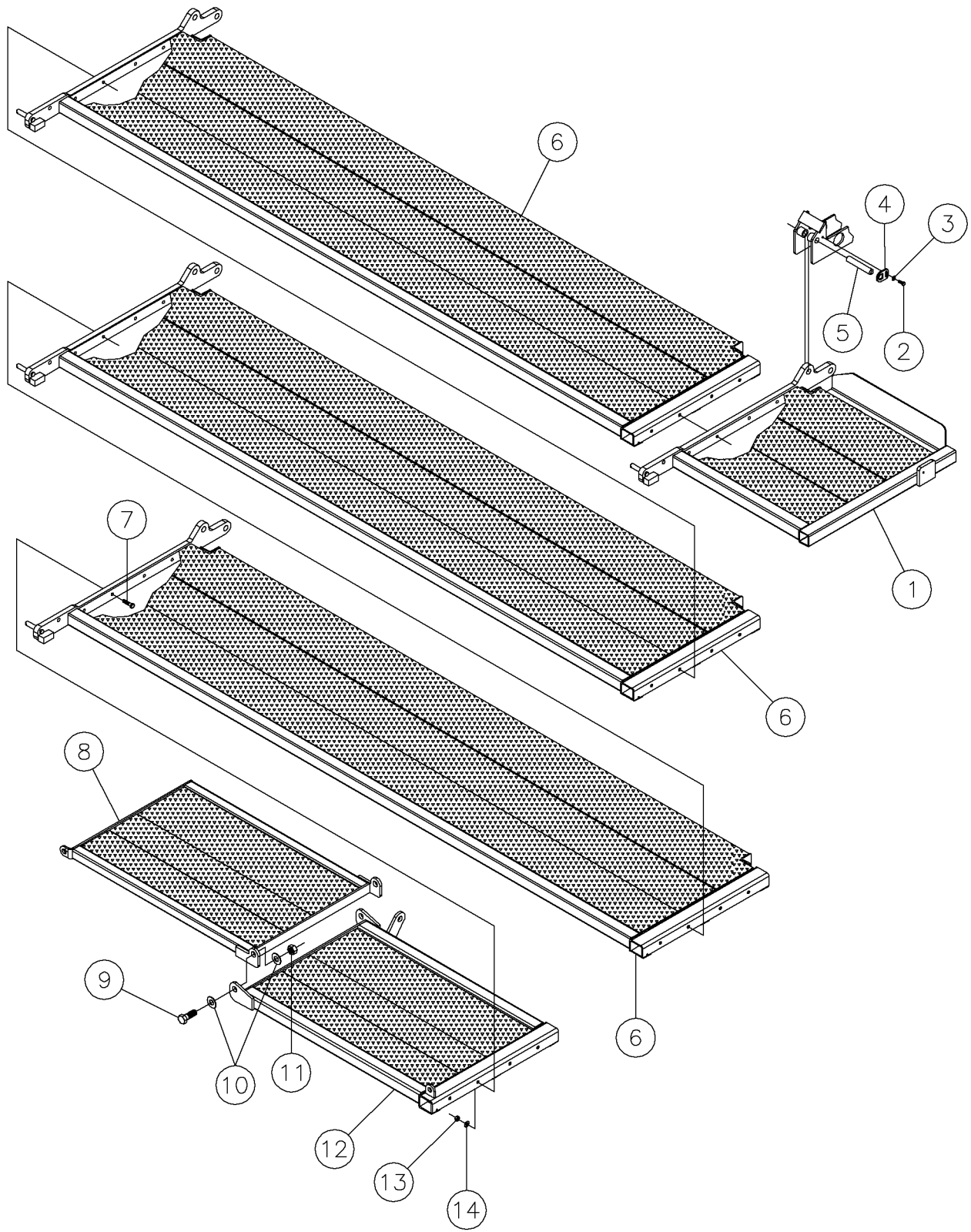
Frame-Catwalk Assy Fig 2-7r02
