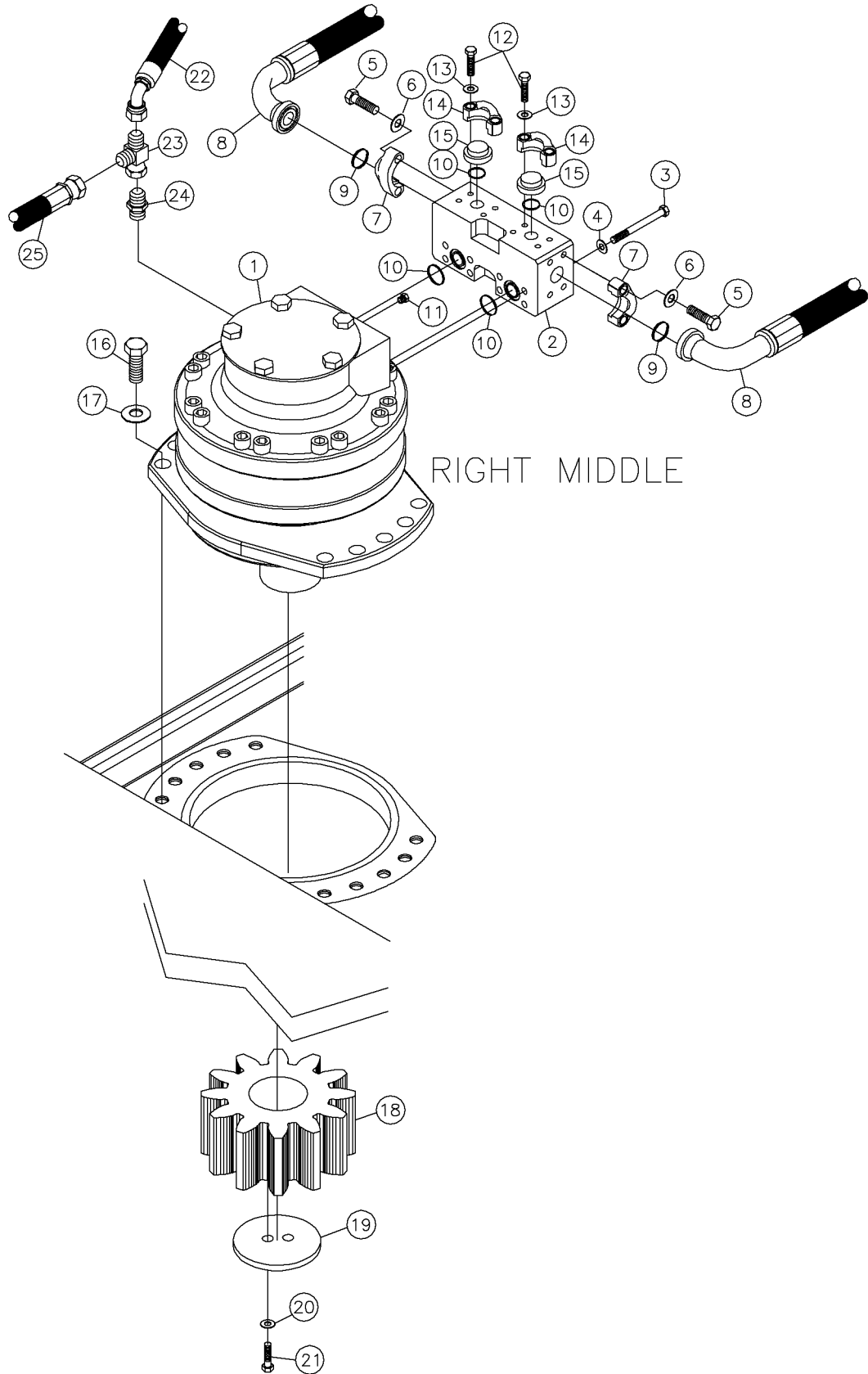
Hyd-Motor-Thrust/Pullback Drive Assy(RM) Fig 5-12x03
