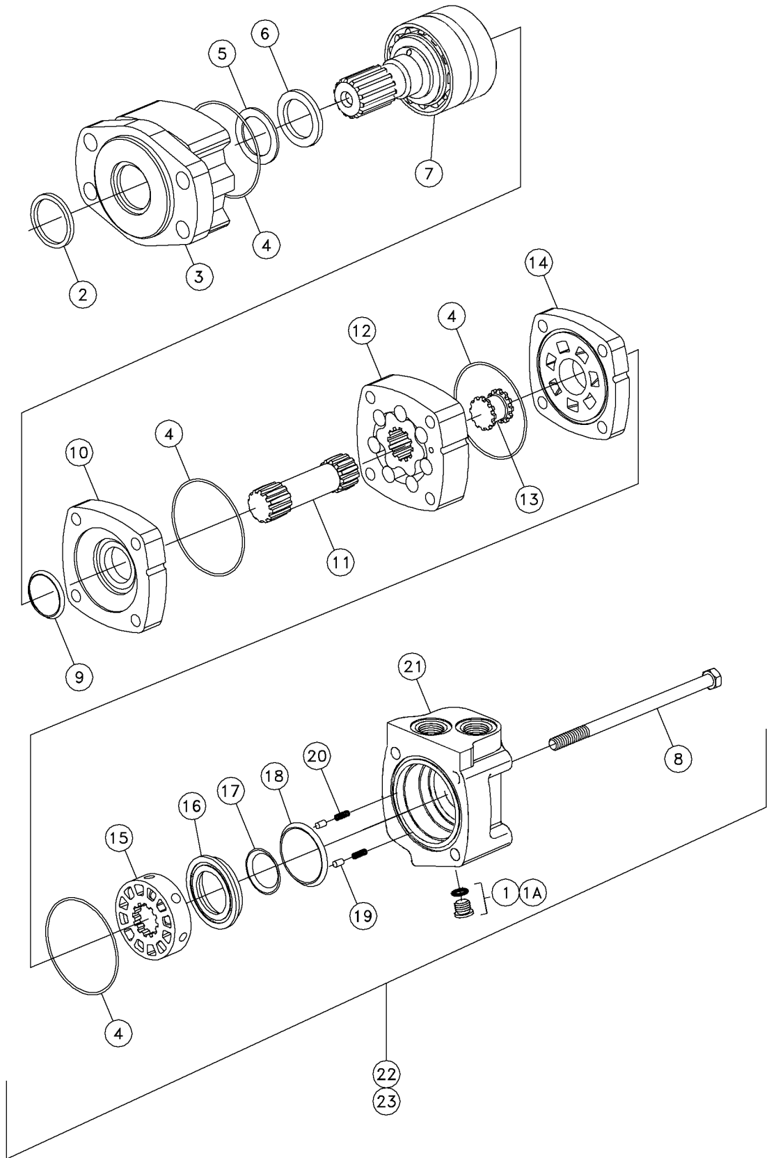
Component-Hyd Motor Fig 12-48
