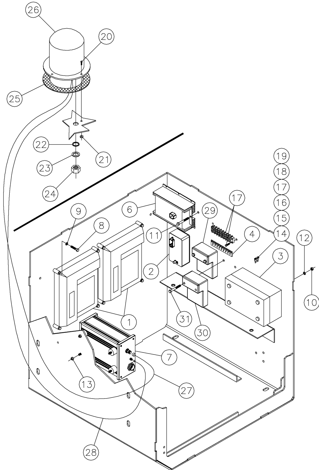
Control/Electrical Box Assy Fig 7-2r01
