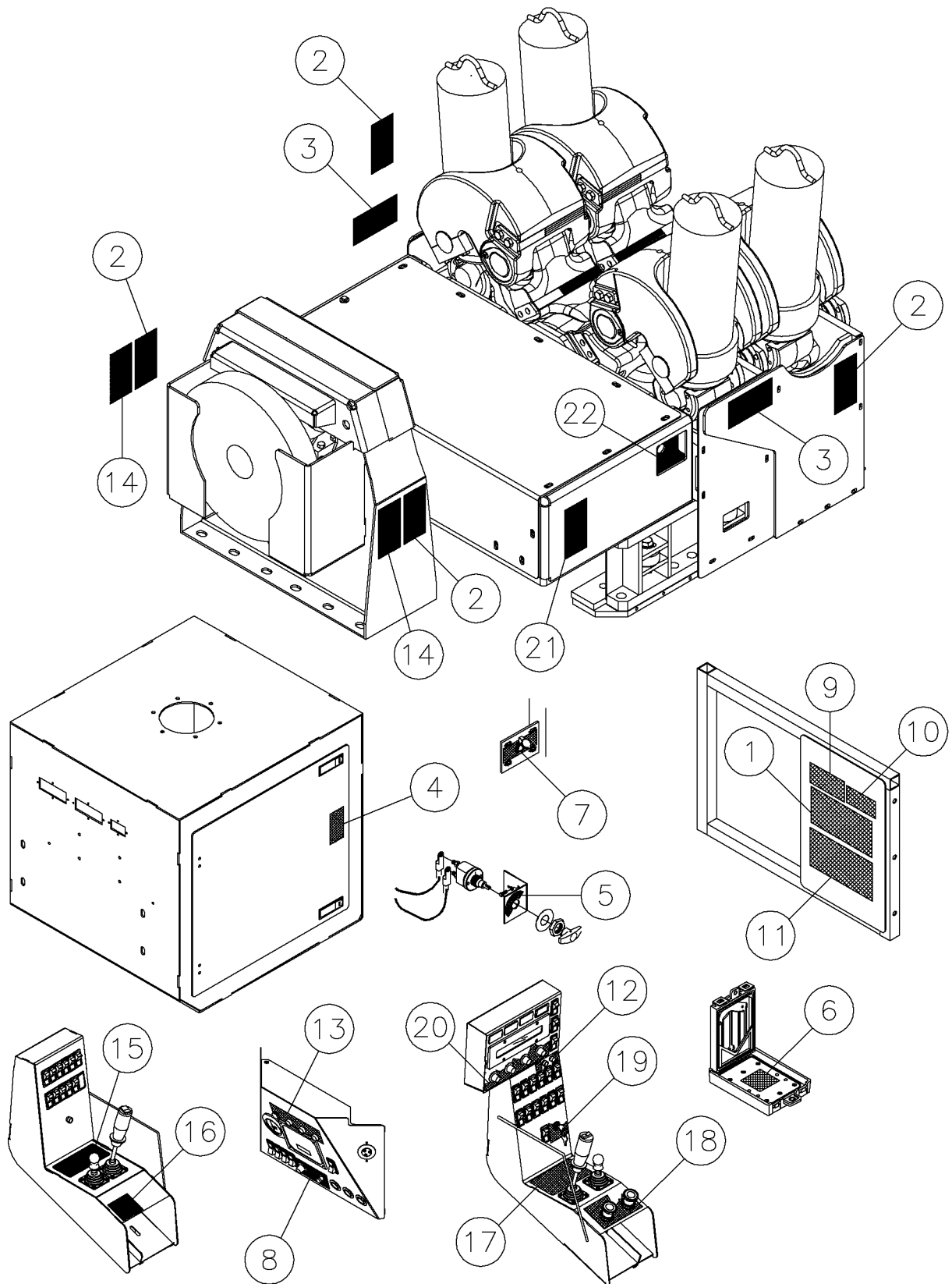
Decal Location Assy-2 Fig 1-4r02
